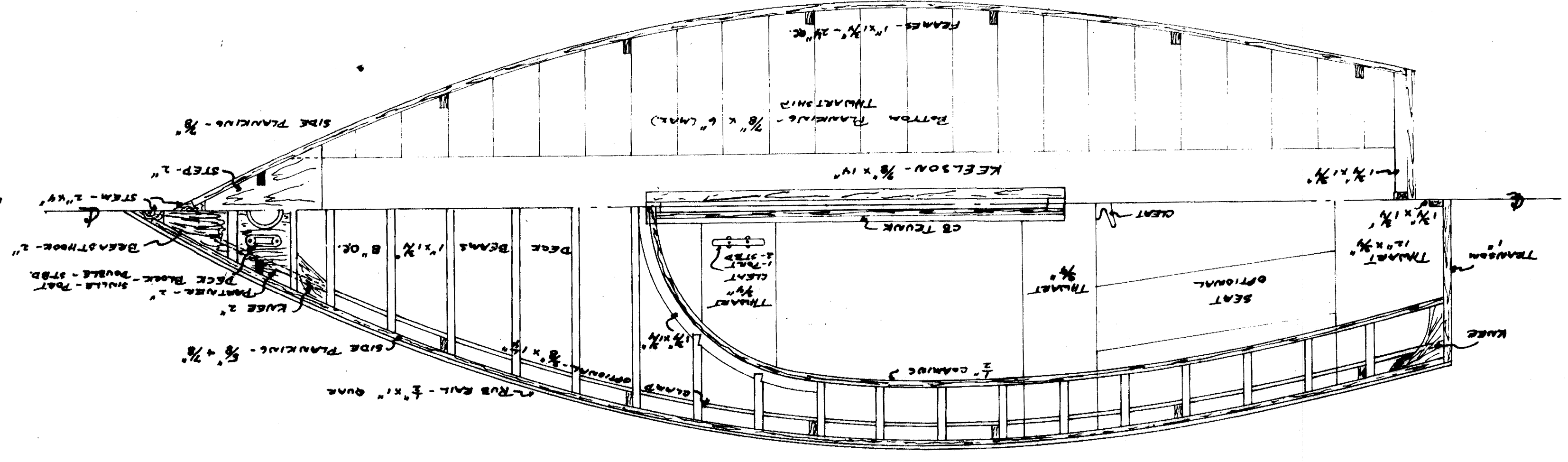
FRAMING HALF PLANS - DECK & BOTTOM SCALE - 1"=1'
