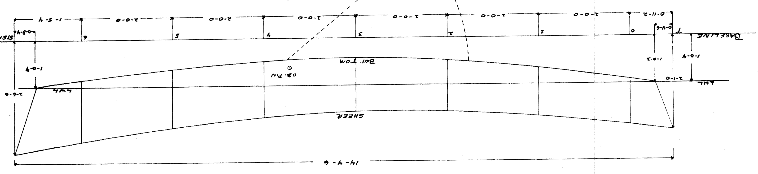
LINES PROFILE SCALE - 1"=1'
